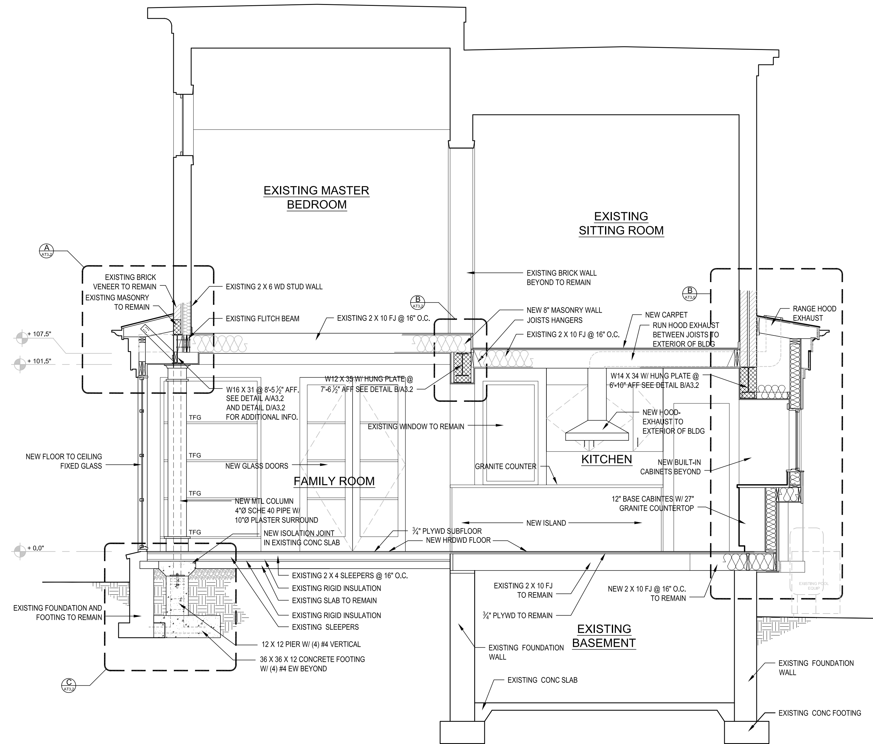
A SECTION C AT3.0 SCALE: 1/4" = 1'-0"
