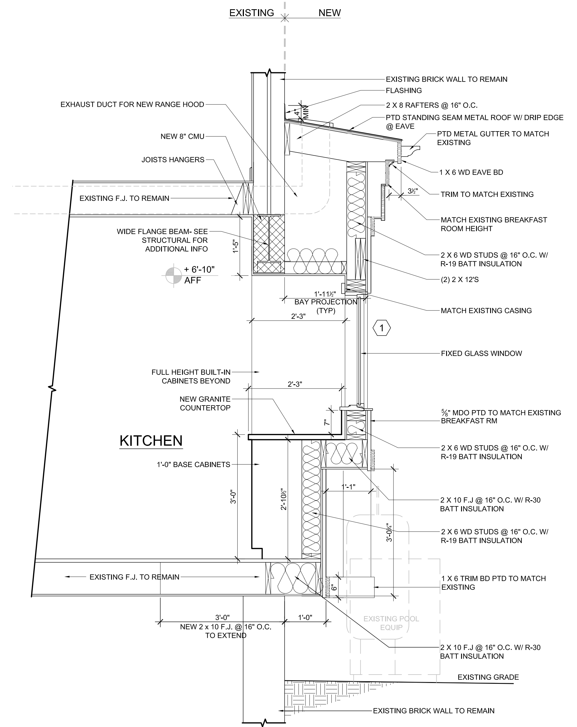
B SECTION D AT3.0 SCALE: 3/4" = 1'-0"
